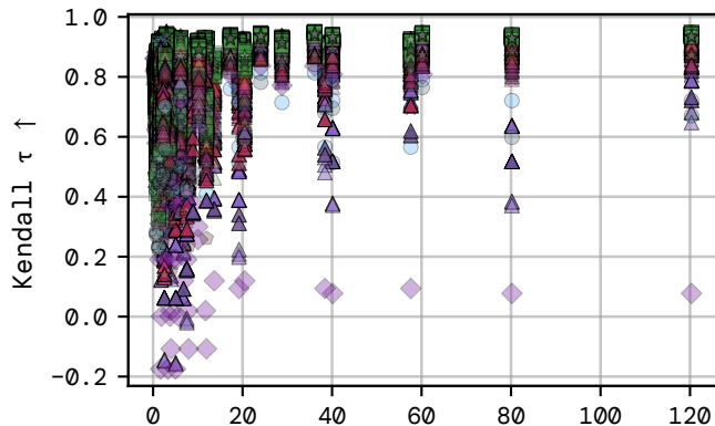
Kendall \tau
